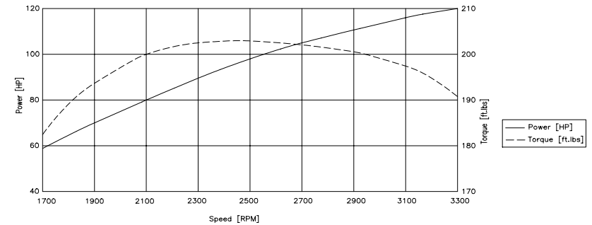
JABIRU 3300 AERO ENGINE PERFORMANCE CURVE
