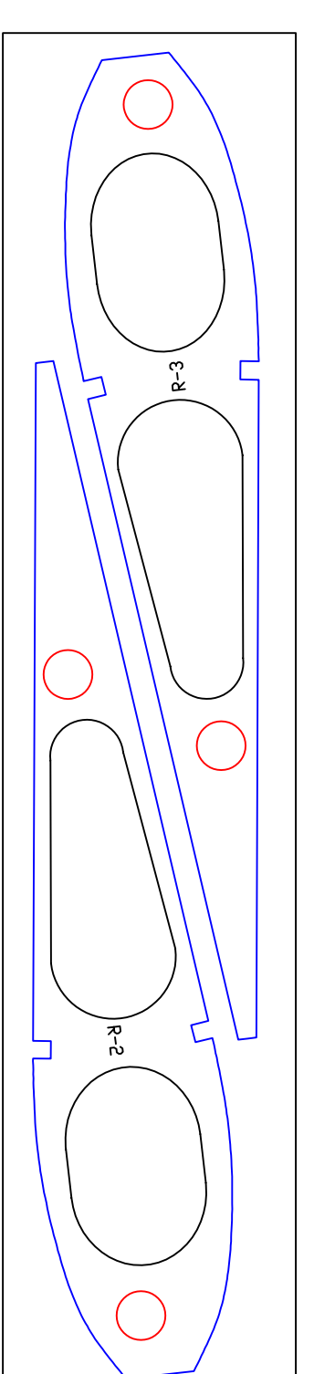
1/8" 1/8" DOUBLE BEVEL RAKE RIB FOR CUTTING LATERAL FLEXURE DO NOT CUT ON SECTION NUMBER REQUEST RIB NUMBER
